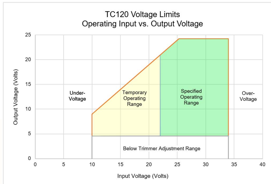
Figure 4.2 TC120 Input Voltage vs Output Voltage Range
